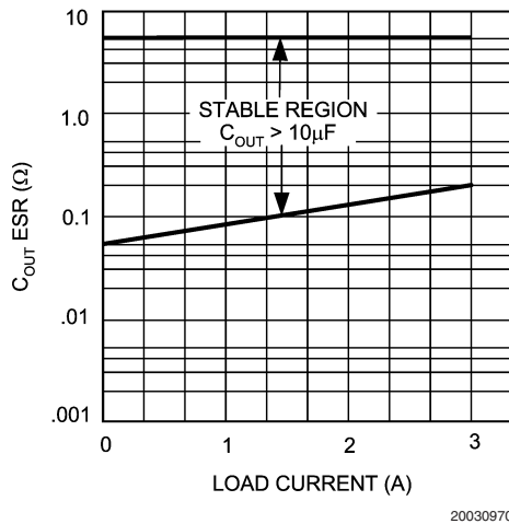
FIGURE 1. ESR Curve for C OUT (with 10 \mu F Tantalum Input Capacitor)
